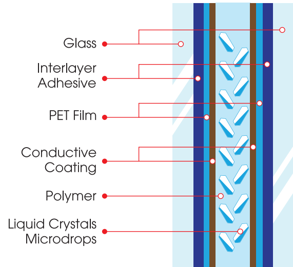
Schematic diagram of the PDLC FILM - based Smart Glass
